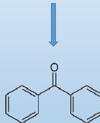
BENZOFENONE
