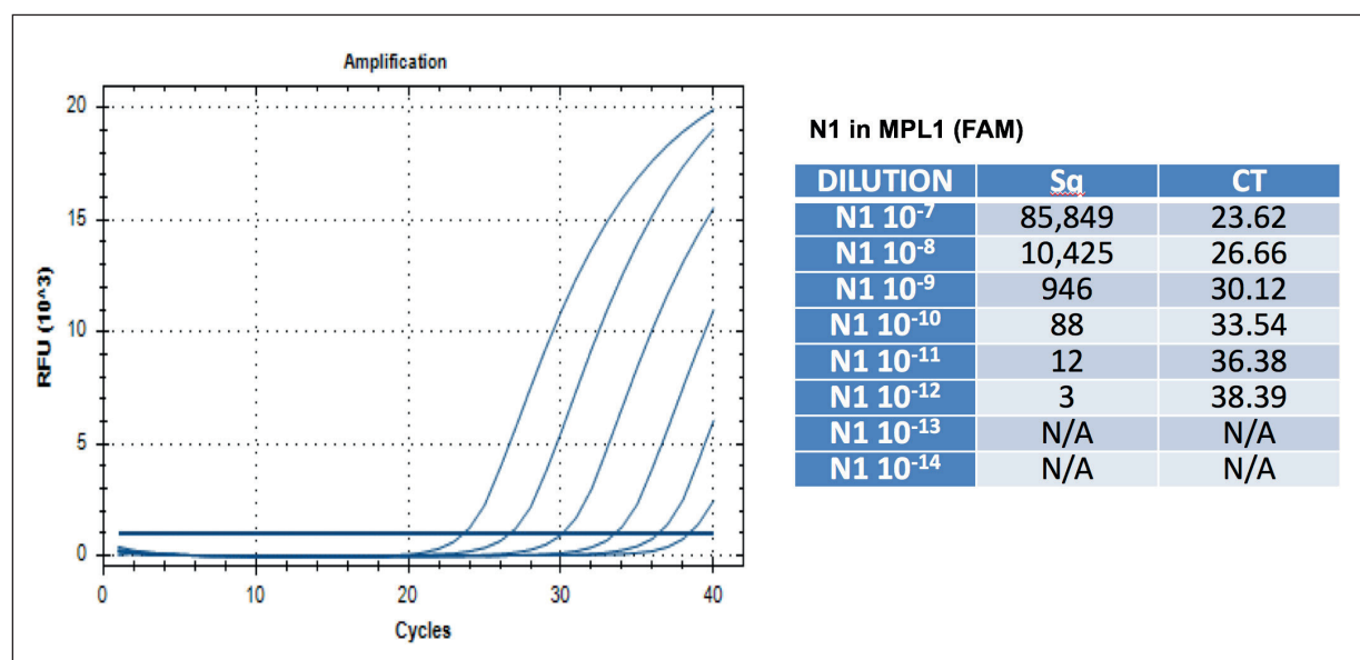
Figure 2. The sensitivity of rRT-PCR step for the detection of N1 gene of SARS-CoV-2.
