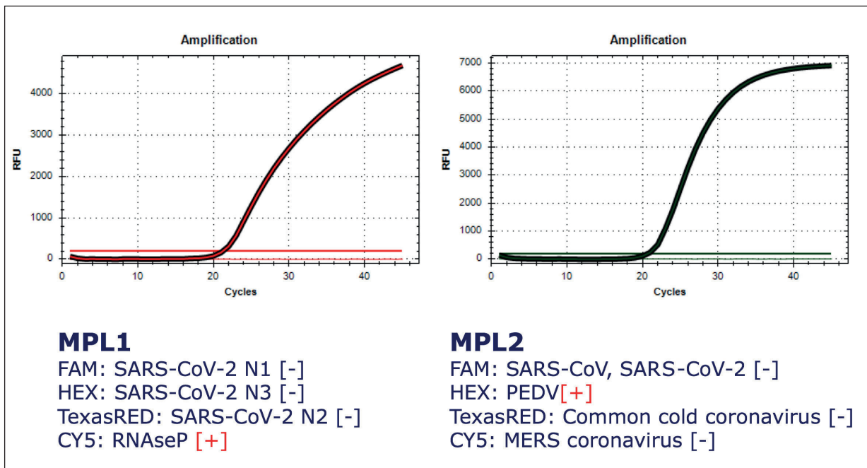
Figure 12. The negative samples with every coronavirus pathogens indicated no amplification of all the related target genes. This result is not false negative, the MLP1 must have the amplification of RP gene (CY5) of the host epithelial cell and the MLP2 must have the amplification of the internal control in the PEDV.
